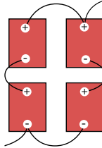
Figure 3 Voltage/Capacity Increase
