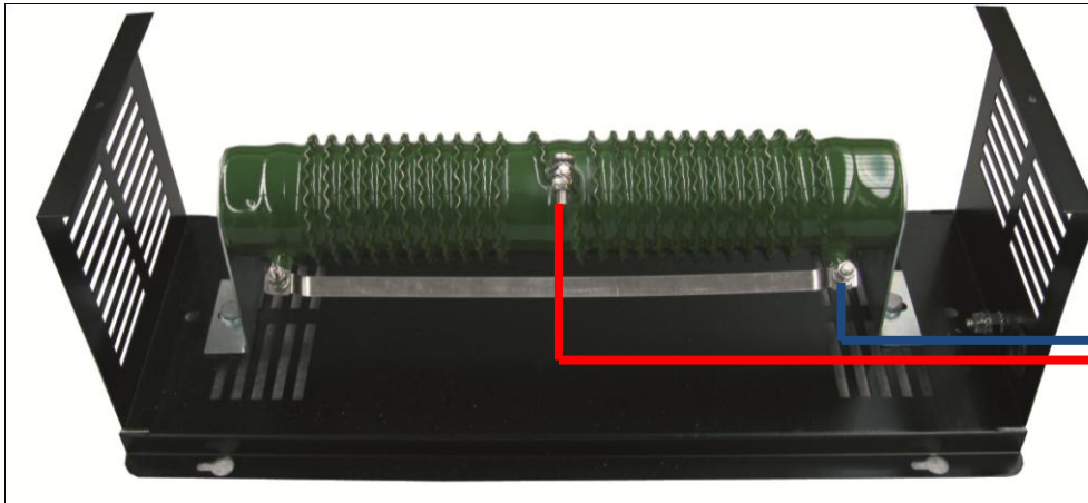
12 Volt x 600 Watt DC Dump Load, RIS12600
